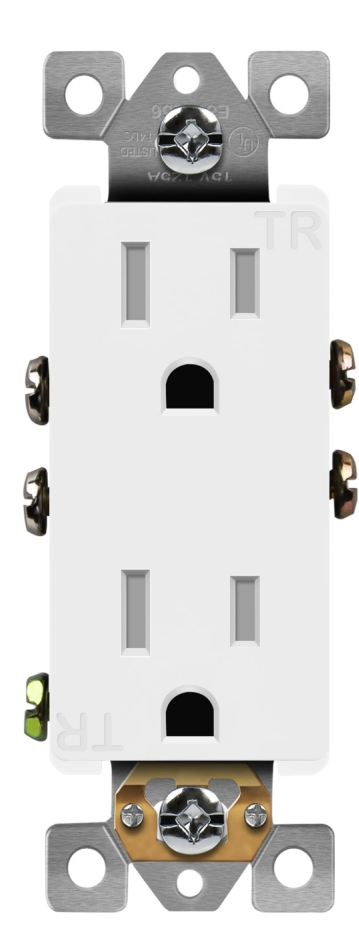
15A/125V Decorator Receptacle SKU: 61501-TR-W
