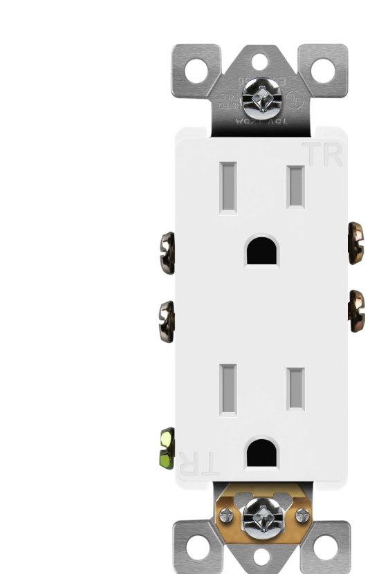
15A/125V Decorator Receptacle SKU: 61501-TR-W LEARN MORE
