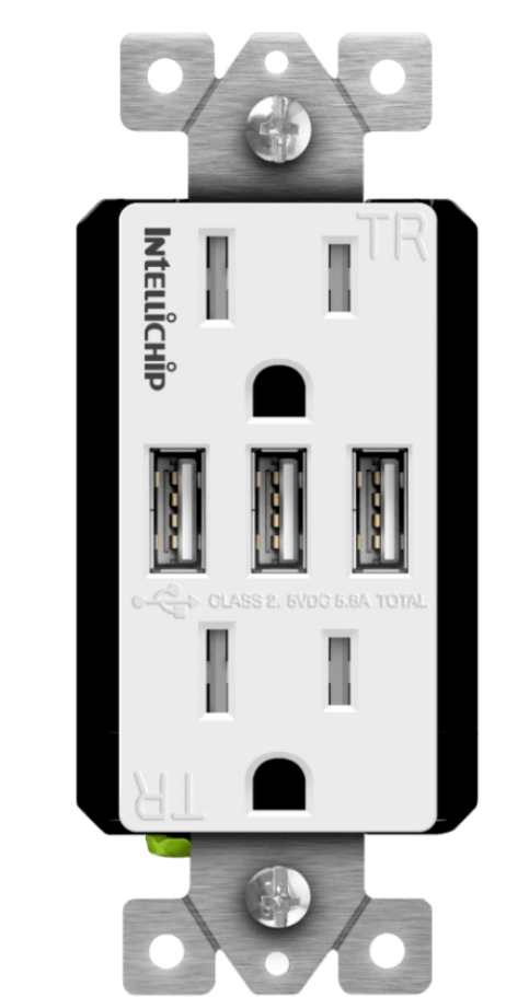
5.8A Triple USB-A Charging Outlet SKU: TU21558A3-W LEARN MORE
