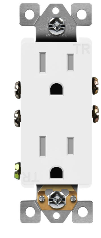
15A/125V Decorator Receptacle SKU: 61501-TR-W LEARN MORE
